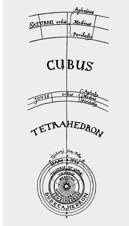
FIGURE 2.1 Kepler's determination of the harmonic ordering of the solar system, from his New Astronomy
